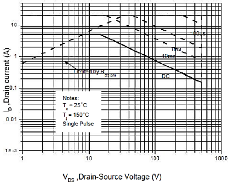
Figure 9. Maximum Safe Operating Area
