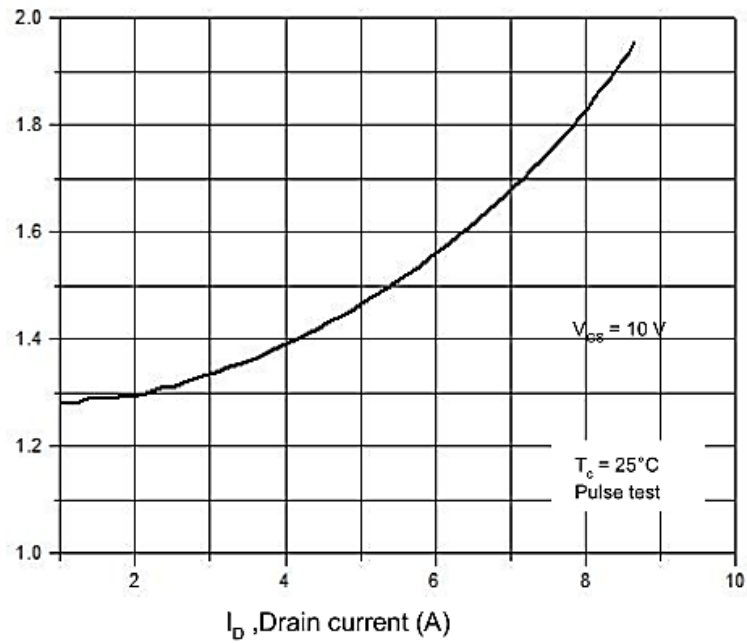
Figure 3. On-Resistance Variation vs. Drain Current
