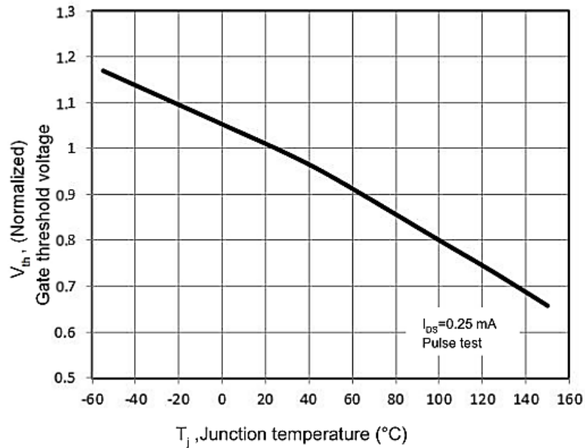
Figure 4. Threshold Voltage vs. Temperature
