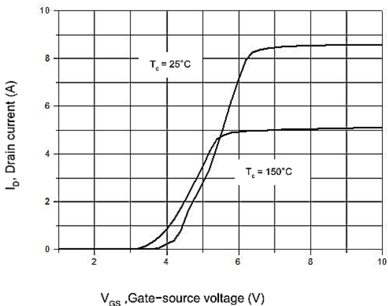
Figure 2. Transfer Characteristics
