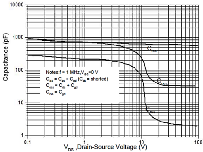
Figure 7. Capacitance Characteristics
