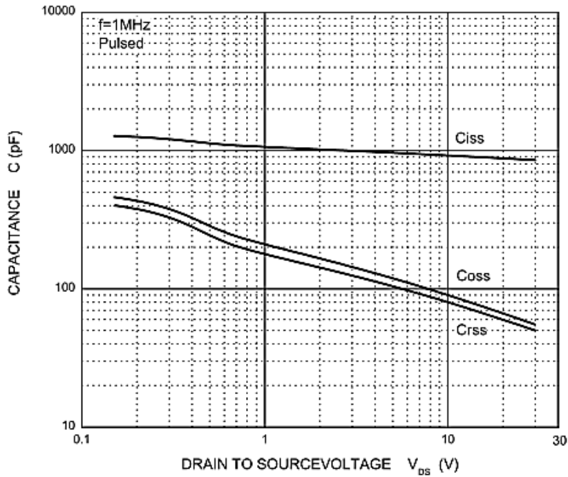
Figure 7. Capacitance Characteristics
