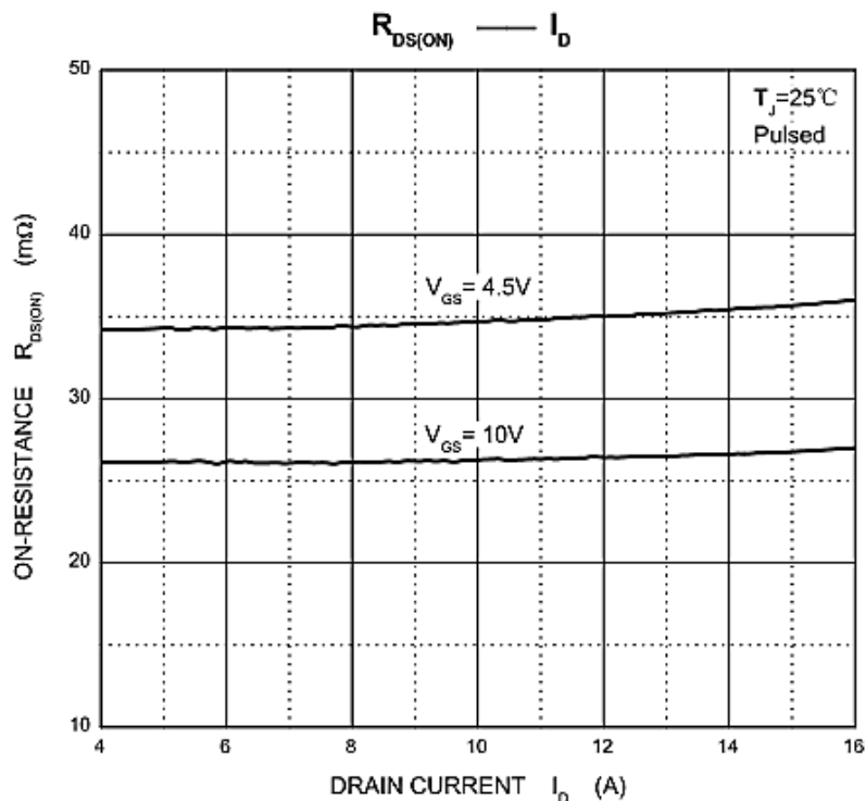
Figure 3. R_{DS(ON)} vs. I_D
