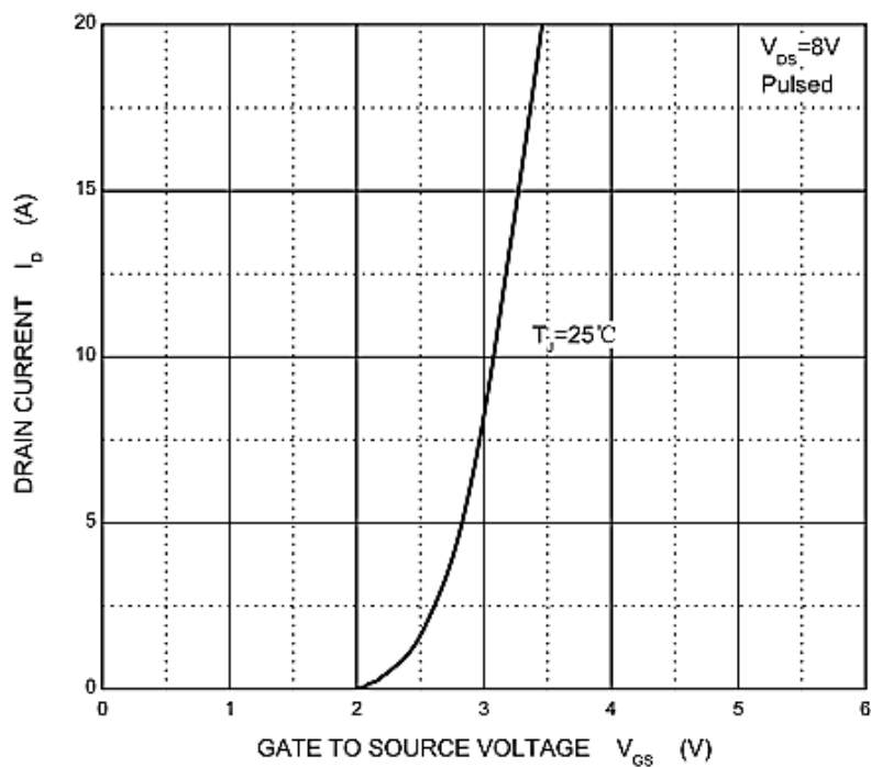
Figure 2. Transfer Characteristics
