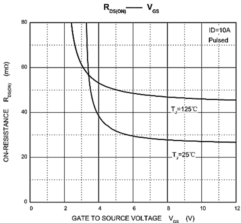
Figure 4. R_{DS(ON)} vs. V_{GS}
