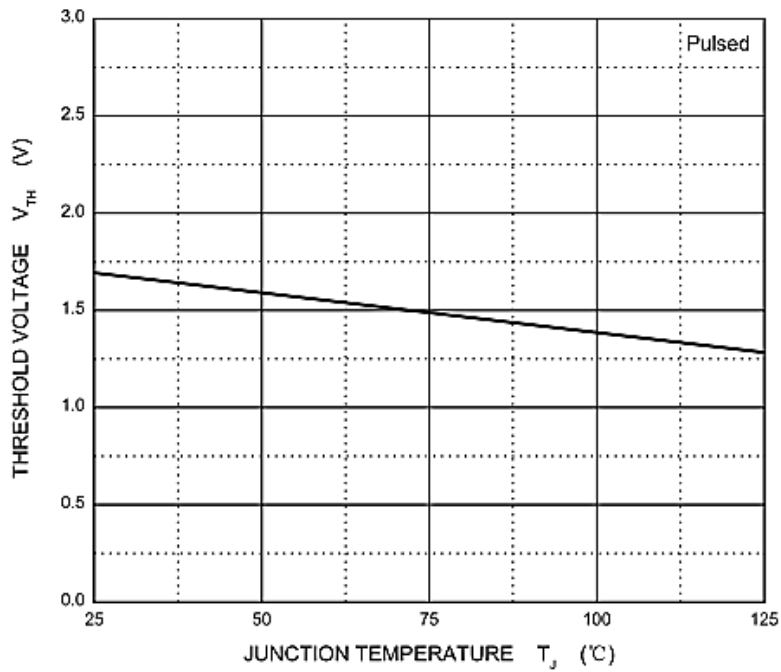
Figure 6. Threshold Voltage vs. Temperature
