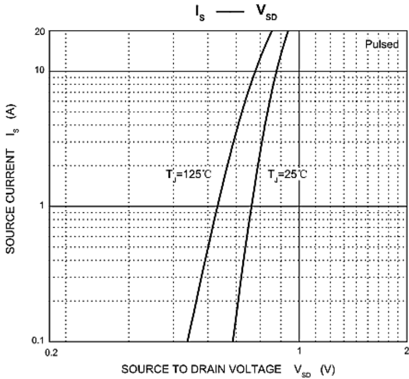
Figure 5. I_s vs. V_{sd}
