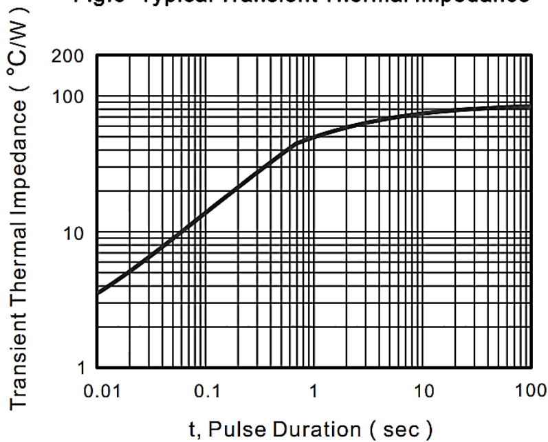
Fig.6- Typical Transient Thermal Impedance
