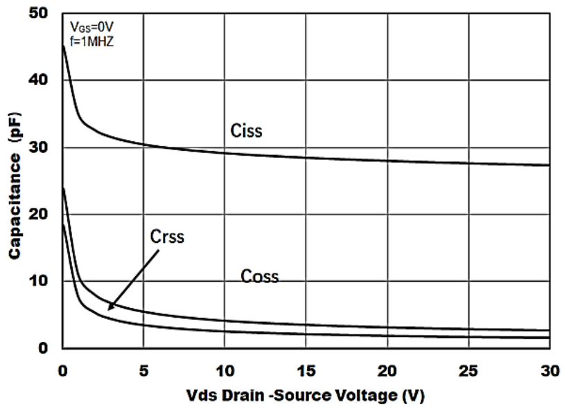
Figure 3. Capacitance Characteristics
