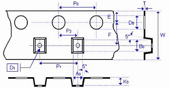
Plastic Tape
