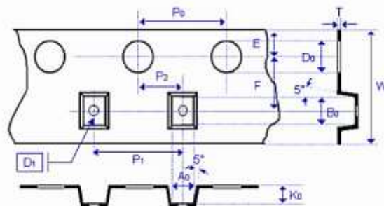
Plastic Tape
