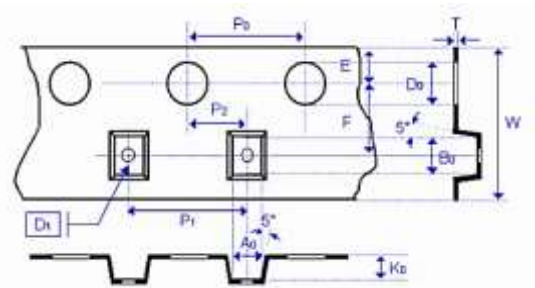
Plastic Tape
