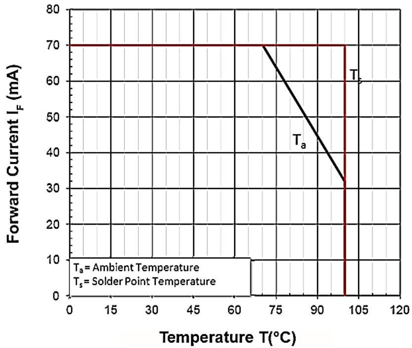
Figure 7 Maximum Current Vs Temperature, I_F = f(T)
