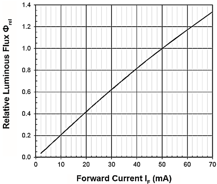
Figure 2. Forward Current Vs. Relative Intensity, \Phi_V/\Phi_V(50mA)=f(I_F)
