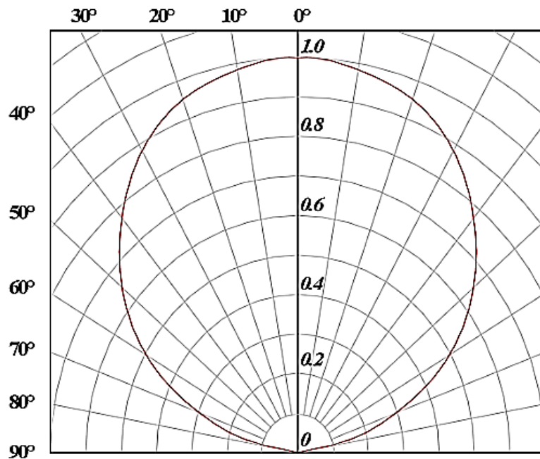
Figure 8. Radiation Diagram, I_{rel} = f(\Phi)
