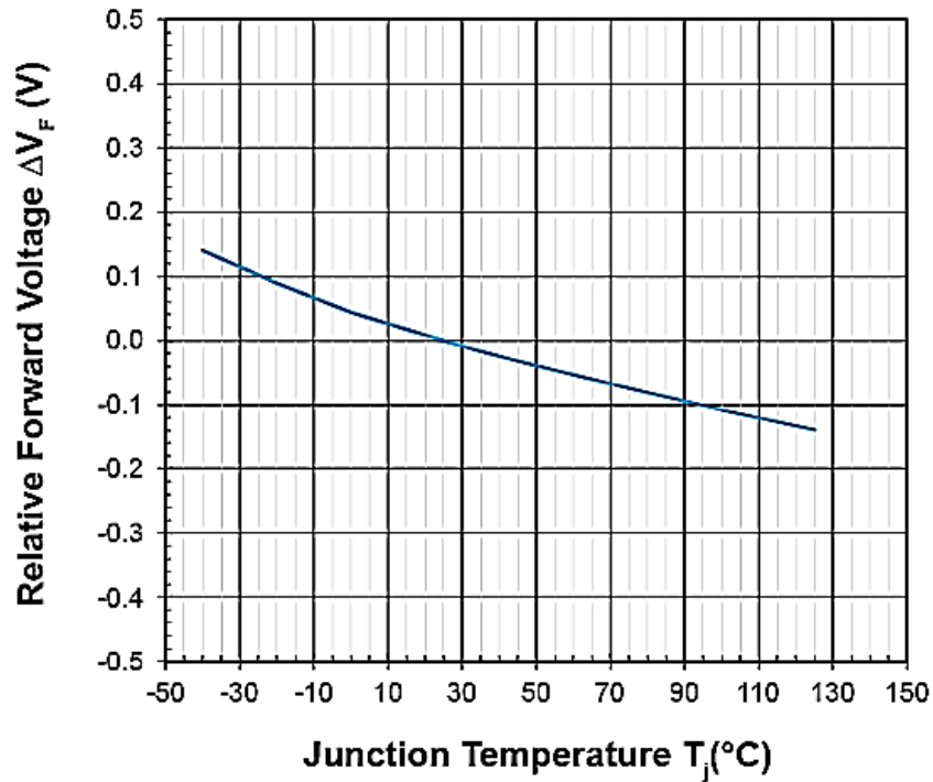
Figure 4. Junction Temperature Vs. Relative Forward Voltage
