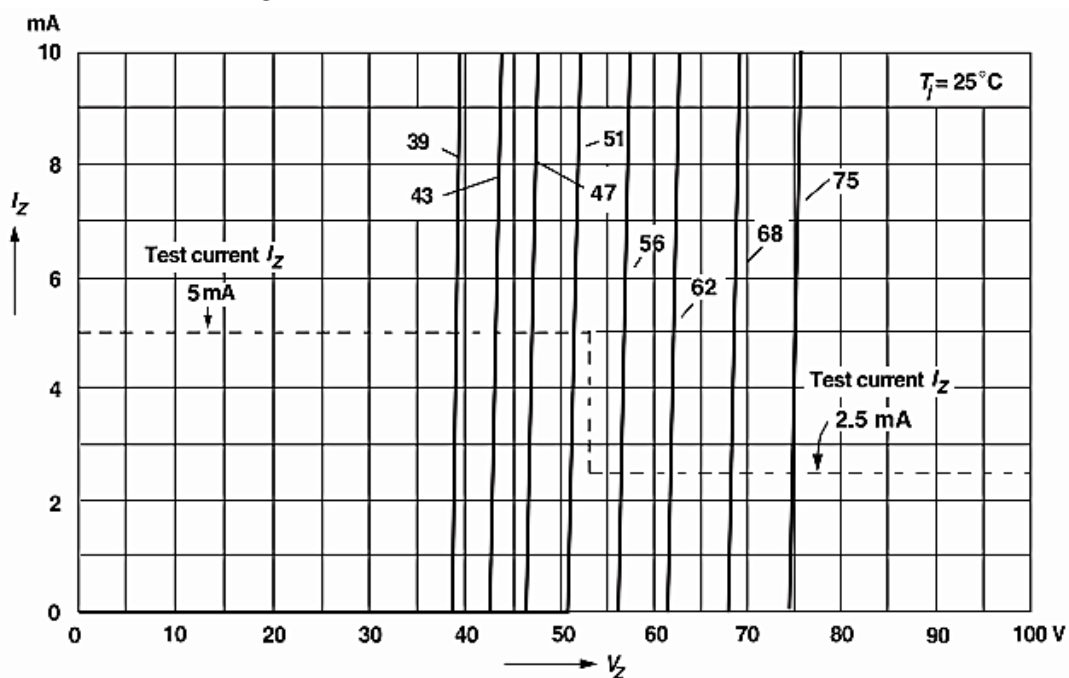
Figure 16. Breakdown Characteristics
