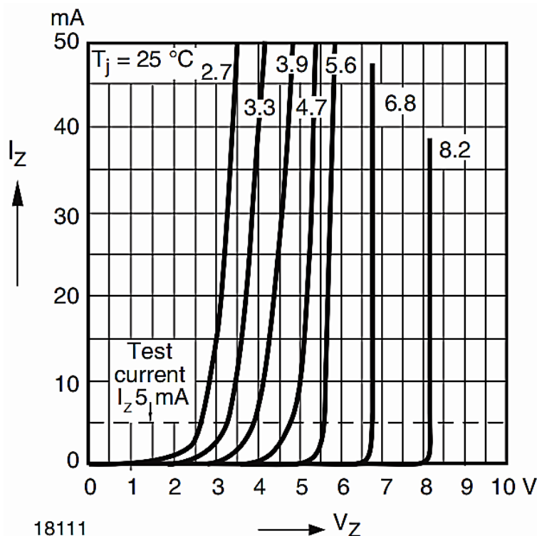
Figure 14. Breakdown Characteristics
