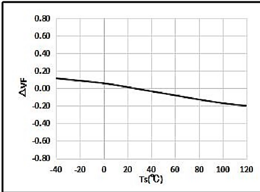
Figure 5. Ts Vs. \Delta V_F
