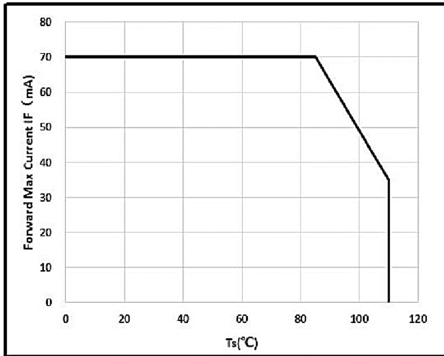
Figure 7 Ts Vs. Max. Permissible IF, I_F = f(T_s)
