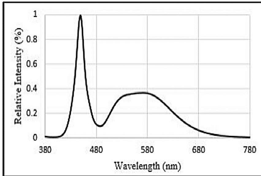
Figure 1. Relative Spectral Emission, I_{rel}=f(\lambda)
