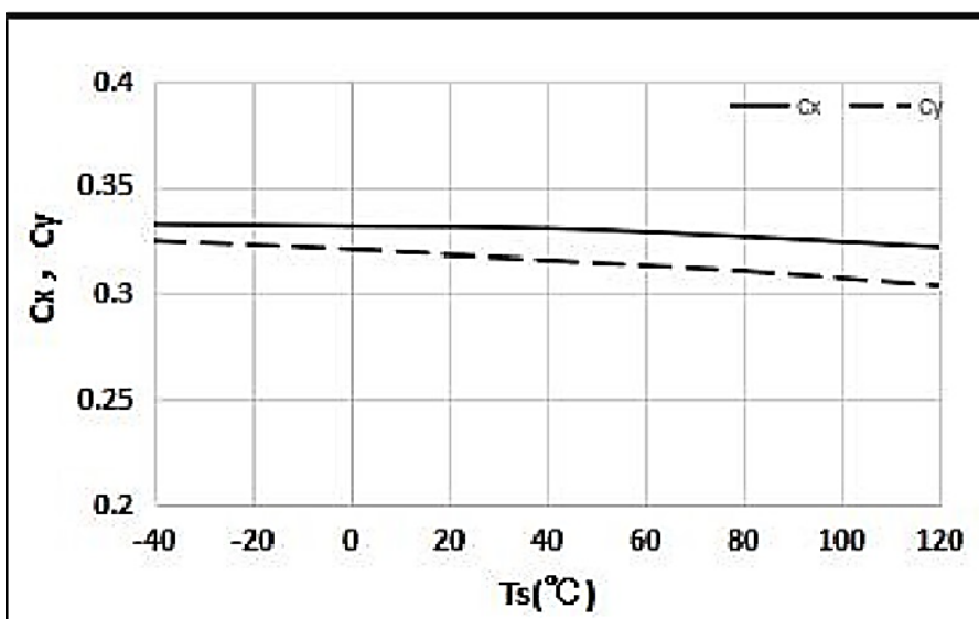
Figure 6. . Ts Vs. Chromaticity Coordinate
