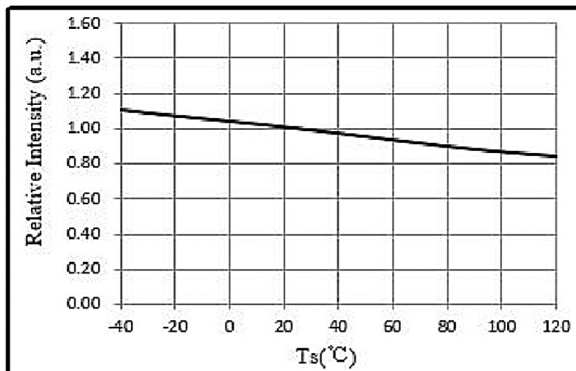
Figure 4. . TS Vs. Relative Intensity
