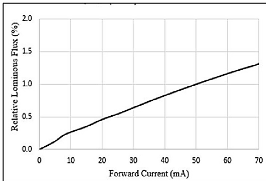
Figure 2. Forward Current Vs. Relative Intensity, \Phi_V/\Phi_V(50mA)=f(I_F)
