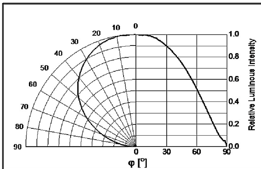
Figure 8. Radiation Diagram, I_{rel} = f(\Phi)
