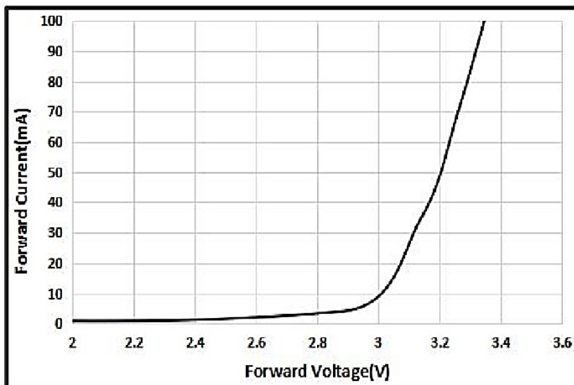
Figure 3. Forward Voltage Vs. Forward Current, I_F = f(V_F)
