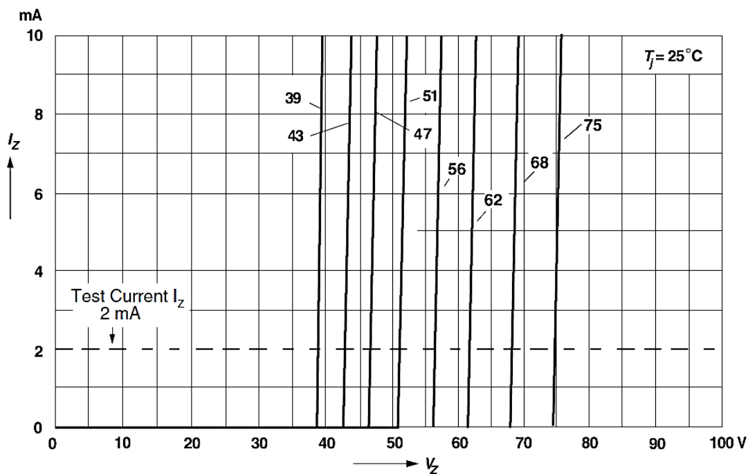
Figure 16. Breakdown Characteristics Curve
