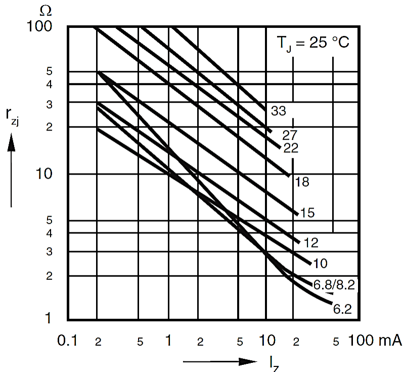
Figure 4. Dynamic Resistance vs. Zener Current Curve
