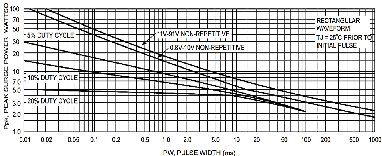
Figure 10. Maximum Surge Power Curve
