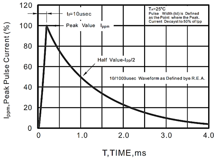
Fig.3 Pulse Waveform
