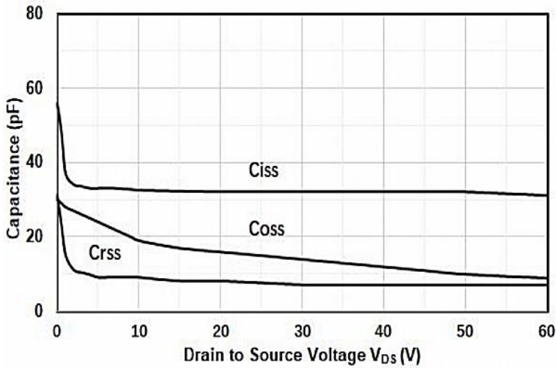
Figure 3. Capacitance Characteristics
